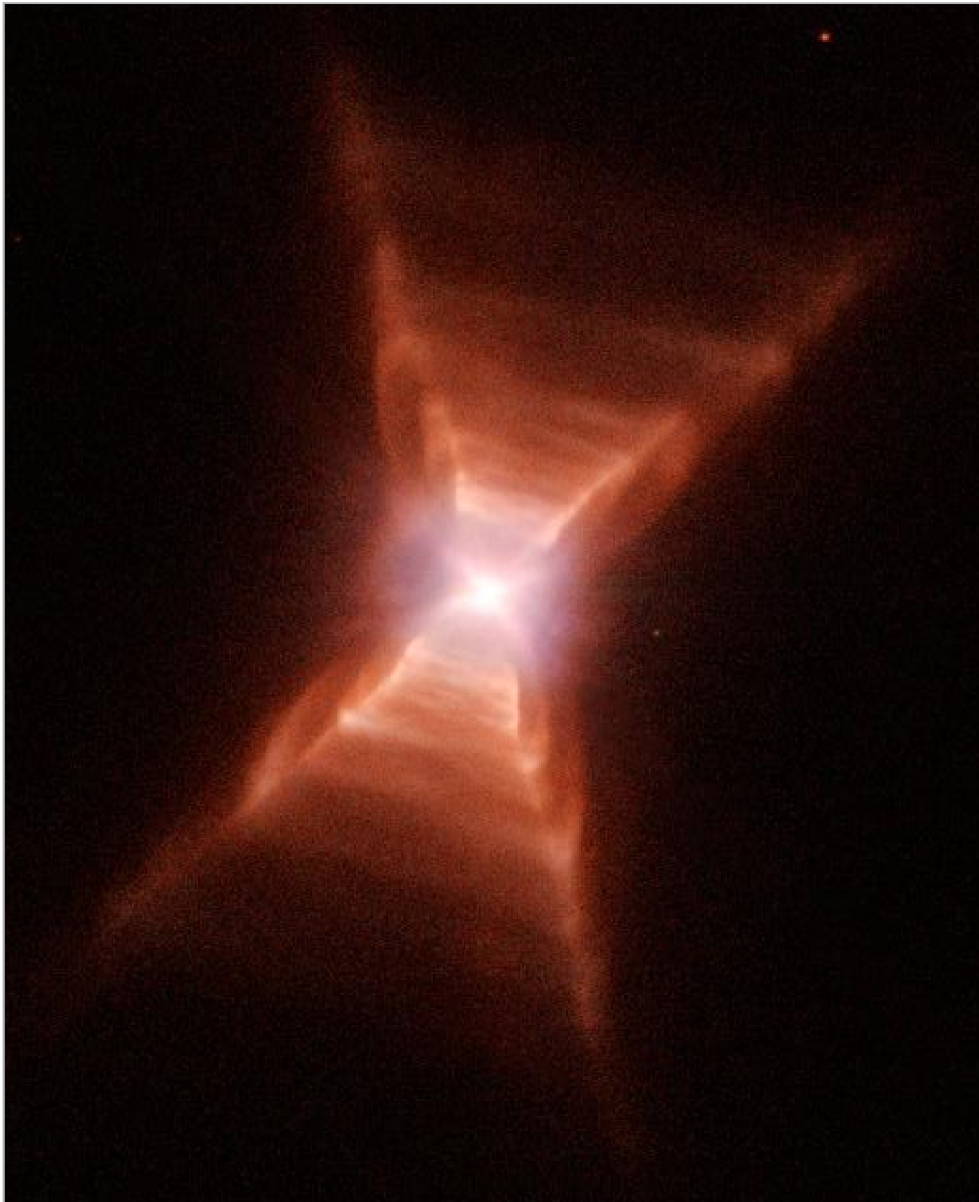
This image, taken with the NASA/ESA Hubble Space Telescope, reveals startling new details in one of the most unusual nebulae known in our Galaxy. Catalogued as HD 44179, this nebula is more commonly called the “Red Rectangle” because of its unique shape and colour as seen with ground-based telescopes.
