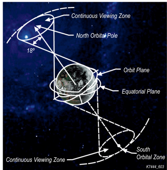
Fig. 6-3 Continuous viewing zone celestial viewing
