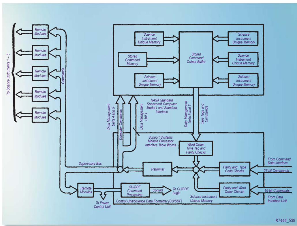
Fig. 5-27 Command flow for Science Instrument Command and Data Handling unit
