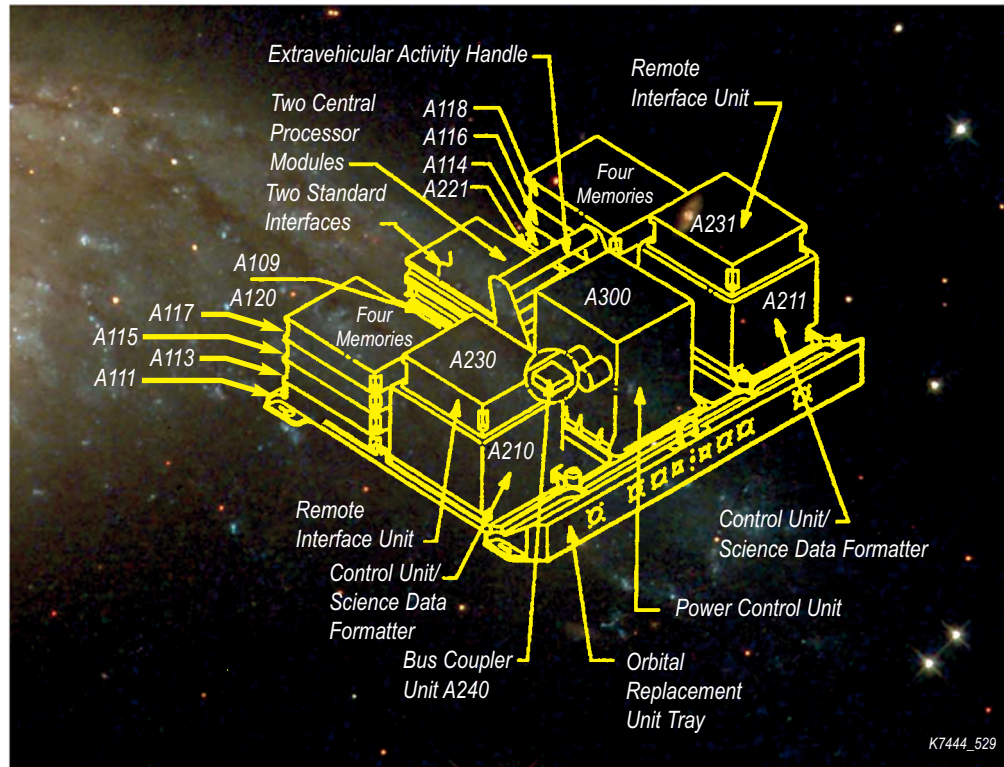
Fig. 5-26 Science Instrument Command and Data Handling unit
