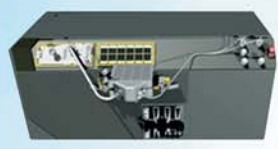
Advanced Camera for Surveys (ACS) repair In Aft Shroud
