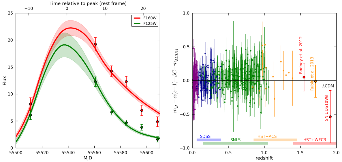
Fig. 4.— On the left, the SALT2 light-curve fit to SN UDS10Wil. SALT2 gives a normal set of light-curve parameters along with a corrected magnitude of 26.15 \pm 0.39 ( 1.4\sigma from \Lambda CDM) and a reduced \chi^2 of 1.5. On the right, we place SN UDS10Wil on the Hubble residual diagram using cosmological parameters from Sullivan et al. (2011) and H_0 = 71.57 \text{ km s}^{-1} \text{ Mpc}^{-1} . For comparison, we also show the compilation of \sim 500 SNe from Conley et al. (2011). Lastly, we include the other two SNe Ia with spectroscopic evidence for classification discovered at a redshift greater than 1.5 (Rodney et al. 2012; Rubin et al. 2013).
