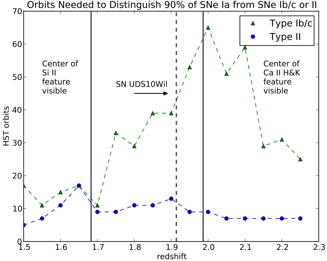
Fig. 5.— The number of orbits necessary to rule out the possibility of a SN II or SN Ib/c when observing a SN Ia. Using aXeSim, we simulated a variety of exposure times in the redshift range 1.5–2.3. We found that \sim 10 orbits can rule out a SN II, but that the number of orbits required to rule out a SN Ib/c possibility is much greater. The number of orbits to rule out a SN Ib/c is much lower in the region where Si II and Ca II H&K are completely visible. These results indicate the need for photometric evidence in SN Ia classification at high redshift, although the HST grism can also be valuable in determining SN redshifts.
